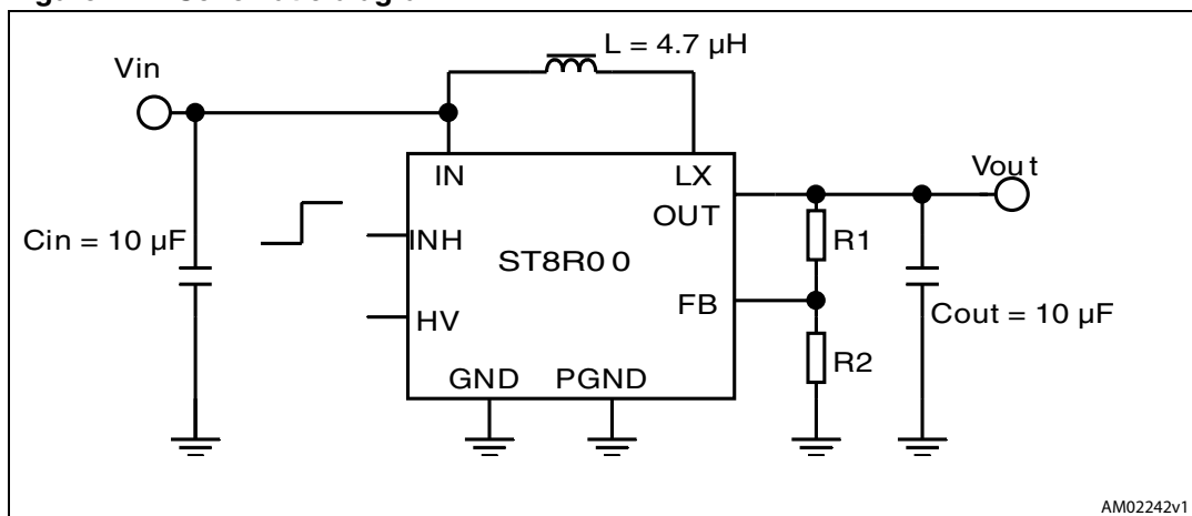
Figure 1. Schematic diagram
